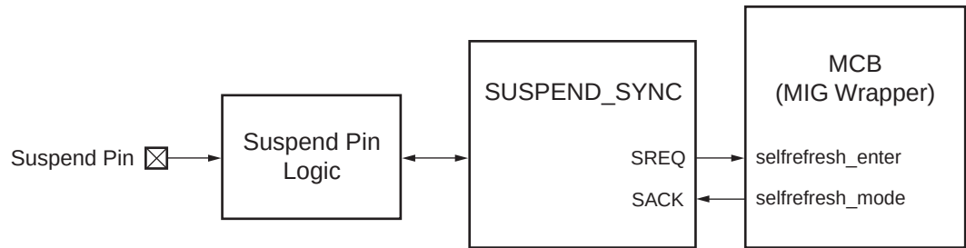
Figure 4-15: SUSPEND_SYNC Connections
