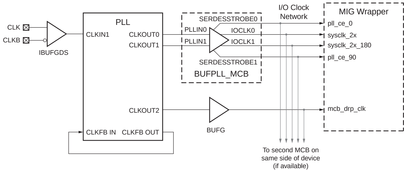
Figure 3-3: Recommended System and Calibration Clock Distribution
