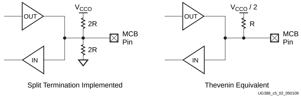
Figure 4-2: Calibrated Input Termination
