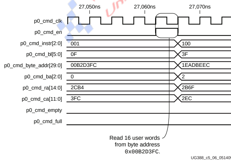
Figure 4-5: Command Path Timing (Read)
