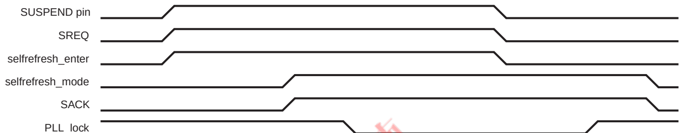
Figure 4-16: Suspend Mode Timing Diagram
