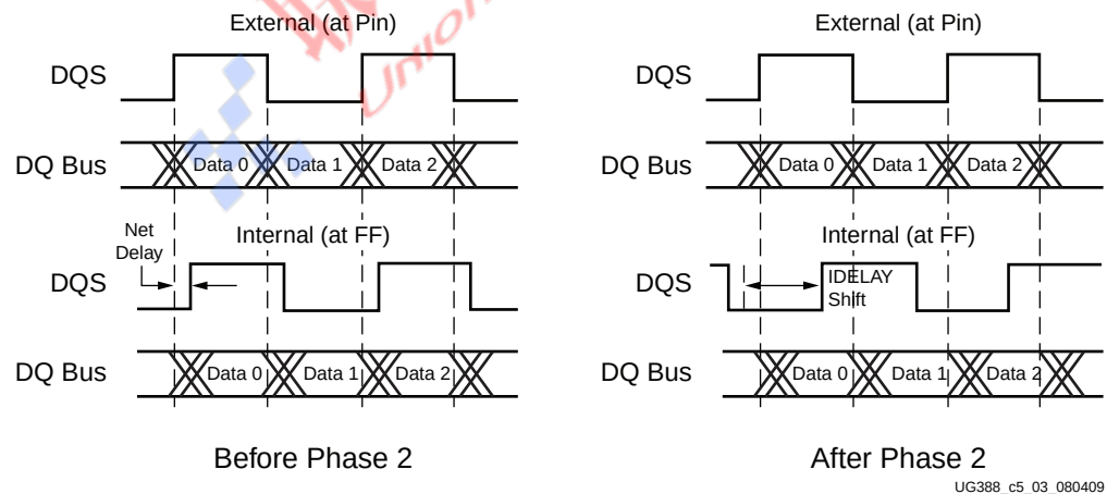
Figure 4-3: Phase 2 of Calibration - DQS Centering
